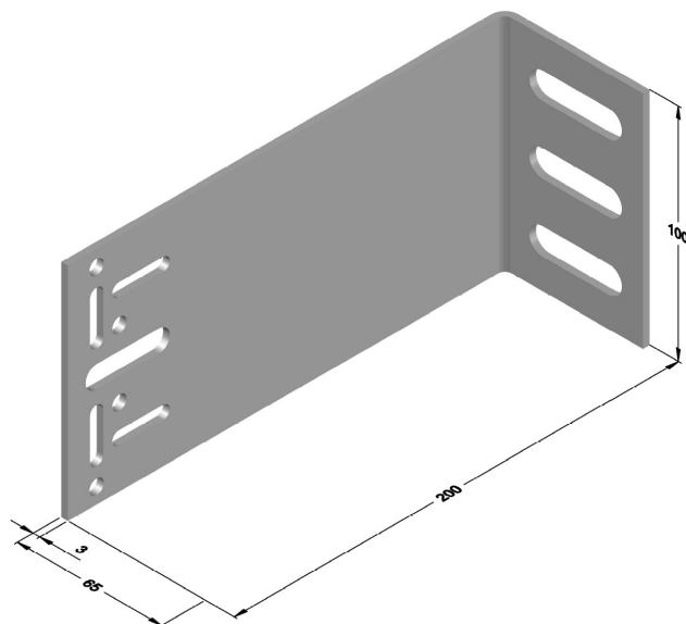
LCFV System Bracket S100
