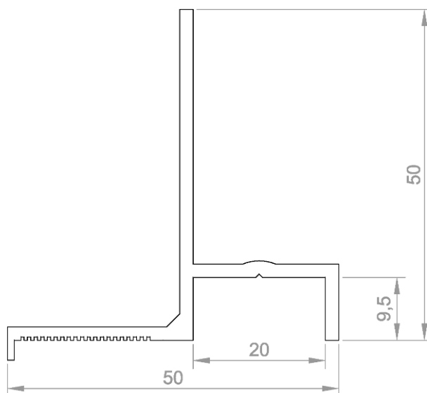
LCFV System Profile L
