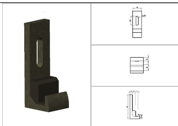
LCFV System Clamp IF/L
