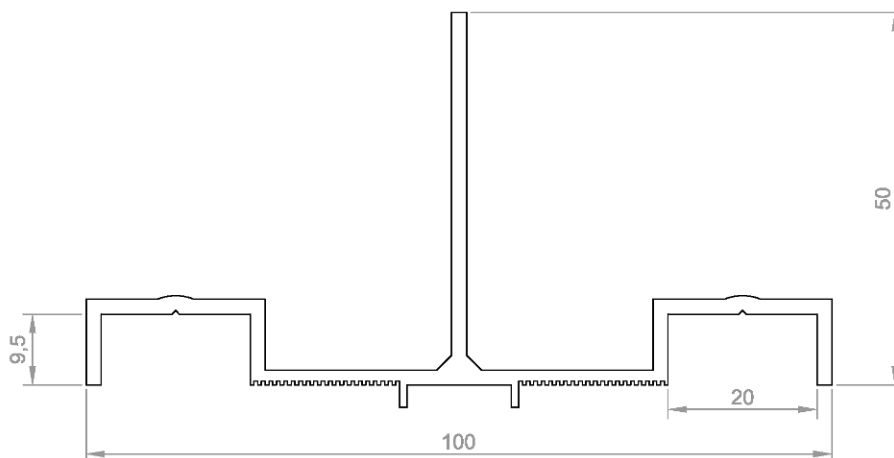
LCFV System Profile T
