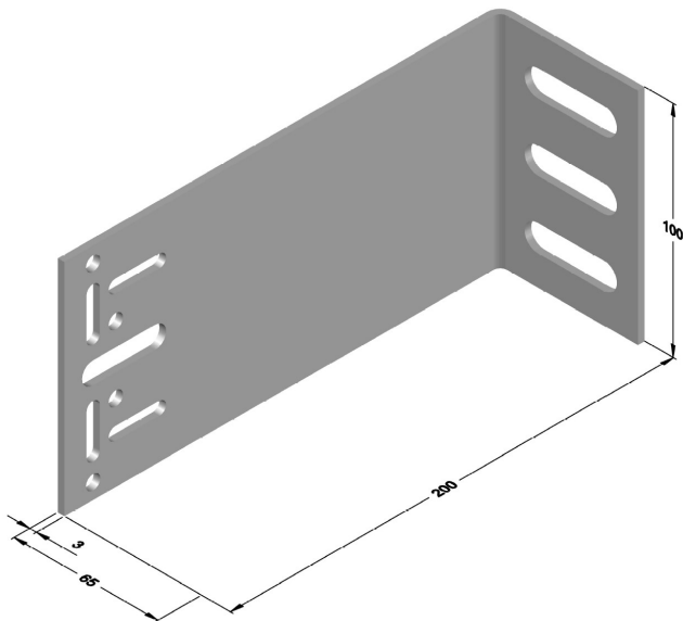
CEXT System Bracket S100
