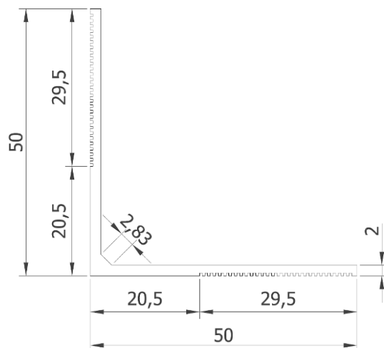
CEXT System Profile L
