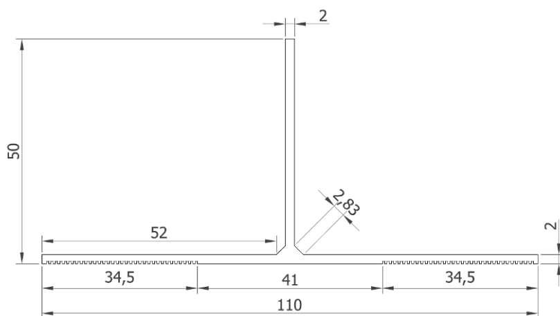
CEXT System Profile T
