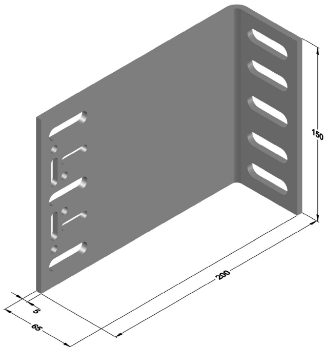
CEXT System Bracket S150
